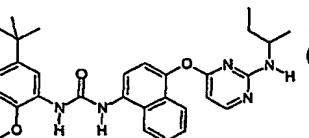
1-[4-(2-sec-Butylamino-pyrimidin-4-yloxy)-naphthalen-1-yl]-3-(5-tert-butyl-2-methoxy-phenyl)-urea;
